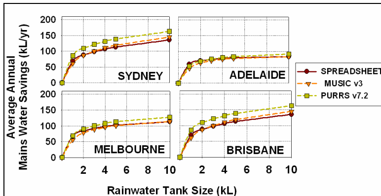
Figure 4: Results from use of climate records of equal duration at each location in models
