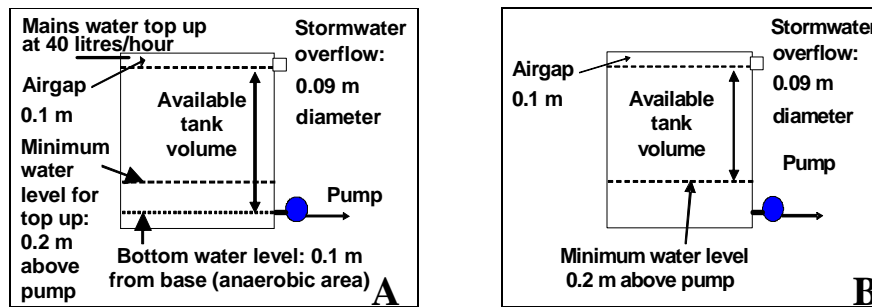
Figure 1: Configuration of tanks used in PURRS (A), and MUSIC and Spreadsheet (B)
