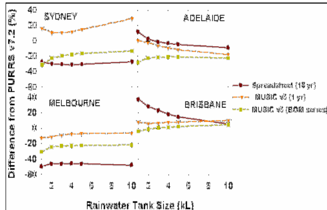
Figure 5: Difference in results from the common use of Spreadsheet and MUSIC in comparison to PURRS results
