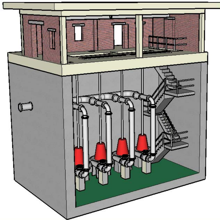
Figure 1: Various views of a pumping station, prepared using Google Sketchup
